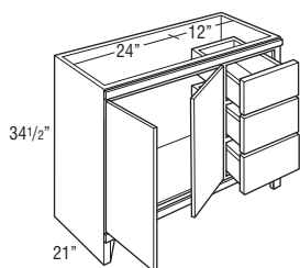
3VSD363421 L or R Butt doors 3VSD363421R shown
