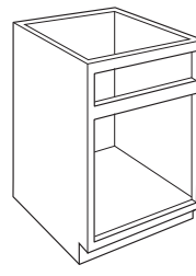
Base cabinets
