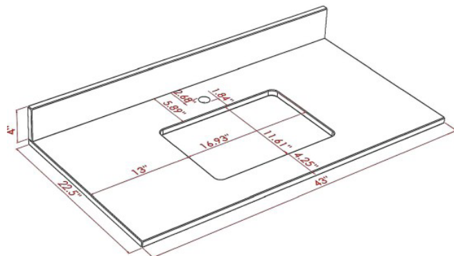
42" VANITY TOP
