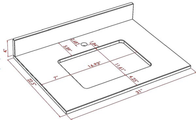
30" VANITY TOP
