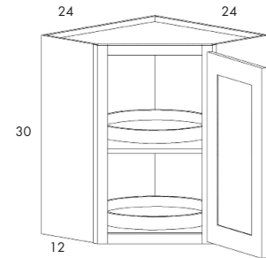
Wall Lazy Susan with Wood Trays (WD)
