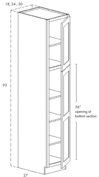
27" Deep Pantry
