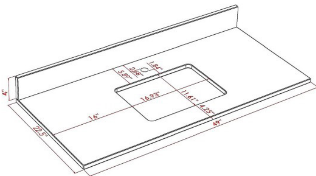
48" VANITY TOP
