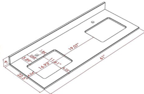
61" VANITY TOP
