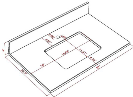
36" VANITY TOP
